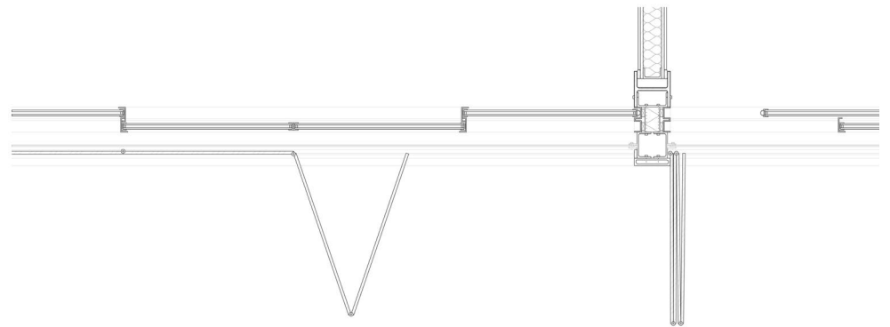
Facade detail section + elevation
