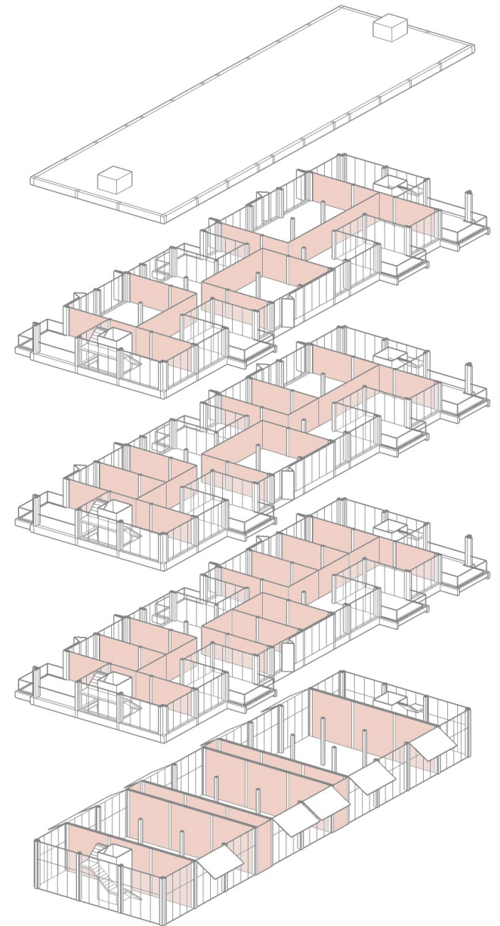
Building levels, exploded view
