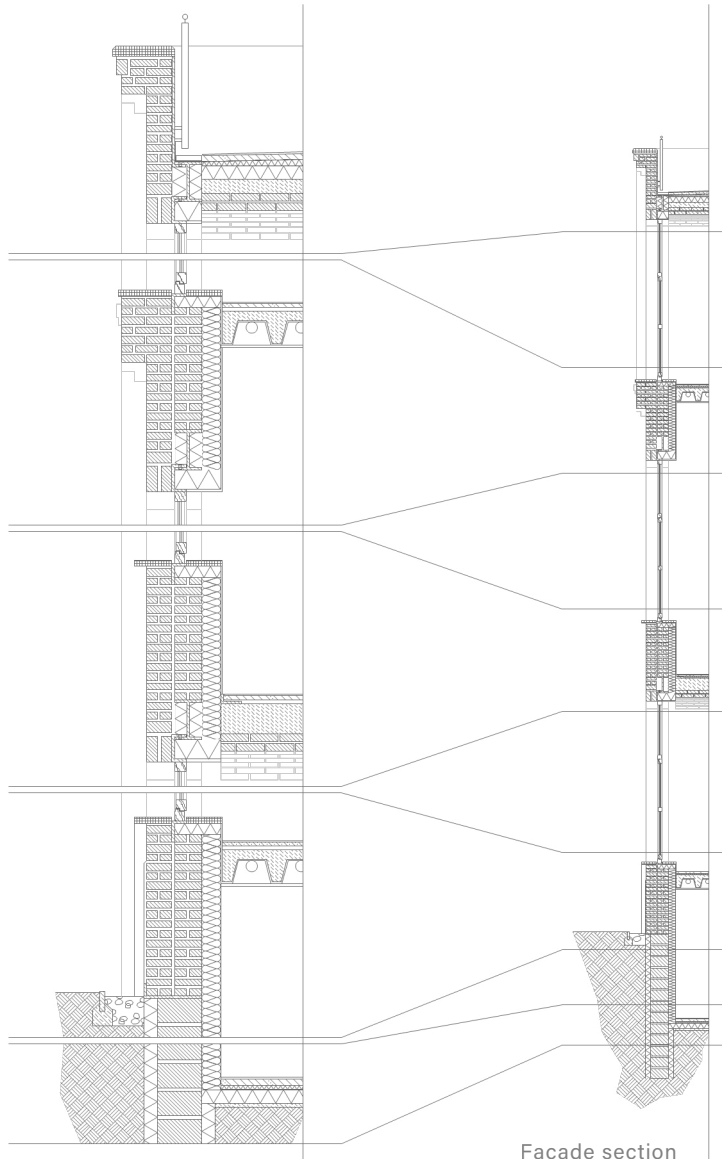
Facade section
