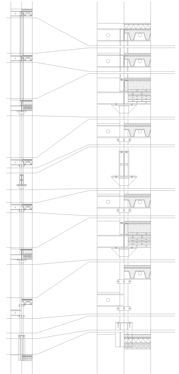
Details pillar
