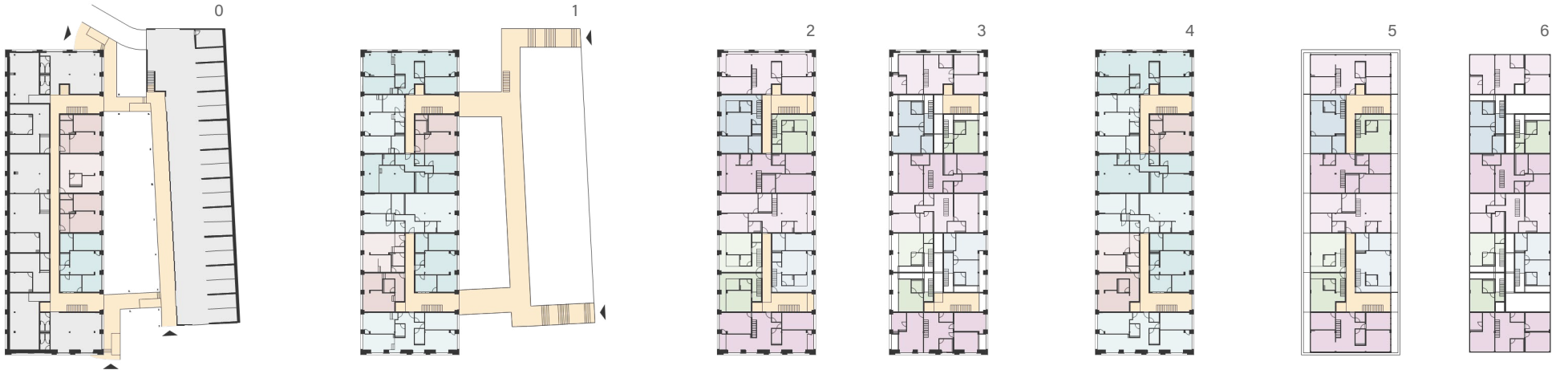
Floor plans
